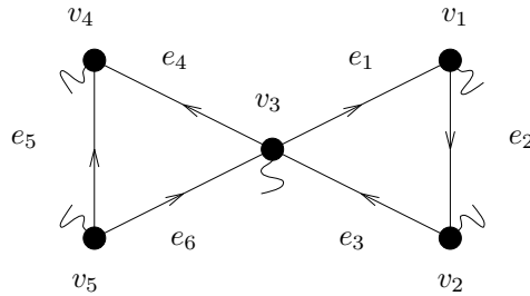
FIGURE 12. Oriented ciliated graph \Gamma .
