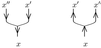
FIGURE 10. Comultiplication acting at a branch.
