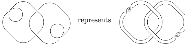
FIGURE 2. Diagram for a framed Hopf link
