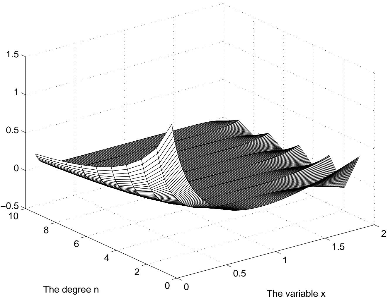
Errors in Taylor polynomial for \log(x)
